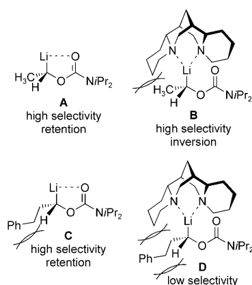
Figure 1. Rationale for the stereochemical outcome considering the steric environment.
