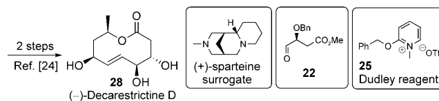
Scheme 4. Synthesis of seco acid 27 : a) SEMCl, DIPEA, CH 2 Cl 2 , 93%; b) LiAlH 4 , THF, 95%; c) ClC(O)NiPr 2 , Et 3 N, CH 2 Cl 2 , 57% (95% brsm); d) (+)-sparteine surrogate, s BuLi, Et 2 O then Bu 3 SnCl, 72%, d.r. > 97:3; e) n BuLi, Et 2 O, then borane 3 , then aldehyde 22 , 85%, ( Z/E > 25:1, anti/syn > 25:1); f) 1. m CPBA, NaHCO 3 , CH 2 Cl 2 then aqueous Na 2 S 2 O 3 ; 2. AcOH, MeOH, 78% (two steps), E/Z > 25:1, anti/syn > 25:1); g) Dudley reagent ( 25 ), MgO, PhCF 3 , 57%; h) LiOH, MeOH/THF/H 2 O (2:2:1), 90%; i) TFA, CH 2 Cl 2 , 77%. Bn = benzyl, brms = based on recovered starting material, DIPEA = diisopropylethylamine, Dudley reagent = 2-benzyloxy-1-methylpyridinium triflate, SEM = 2-(trimethylsilyl)ethoxymethyl, TFA = trifluoroacetic acid.
